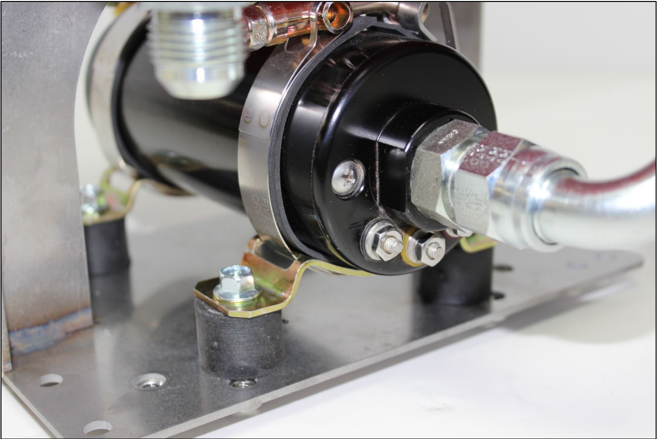
Pump Inlet – ALL #10 (5/8") – Electrical Connections This End – Make Sure to Jumper for REDUCED SPEED!
