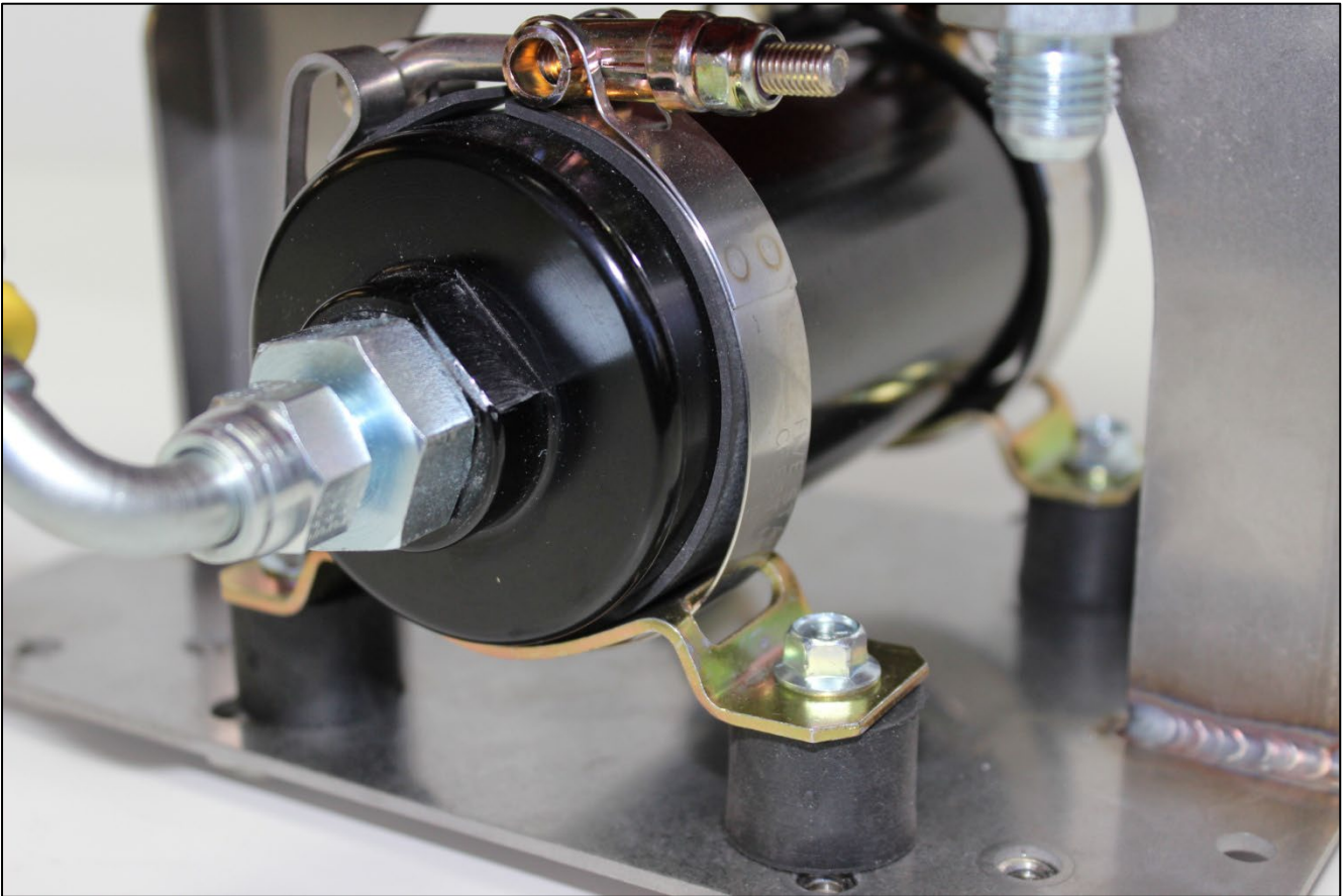
Pump Outlet – ALL #6 (3/8")
